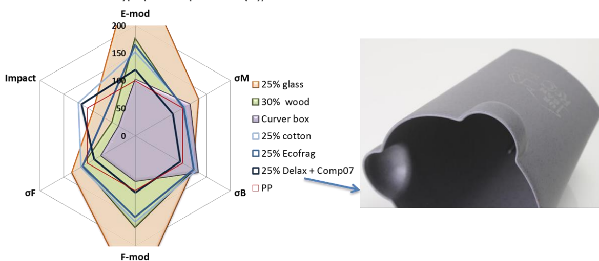
Figure 4 Radar plots comparing the mechanical properties* of the FRC's with cotton, Ecofrag and Delax fibres to virgin PP (left) and illustration of an ice bucket demonstrator produced from the PP-Delax FRC (right).
