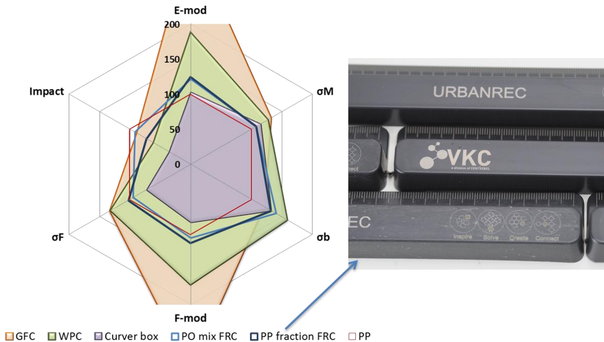
Figure 5 Radar plot comparing the mechanical properties* of the recycled plastics FRC's to unfilled, virgin PP and to virgin WPC and GFC (left) and illustration of the demonstrators produced from the PO mix FRC (right).
