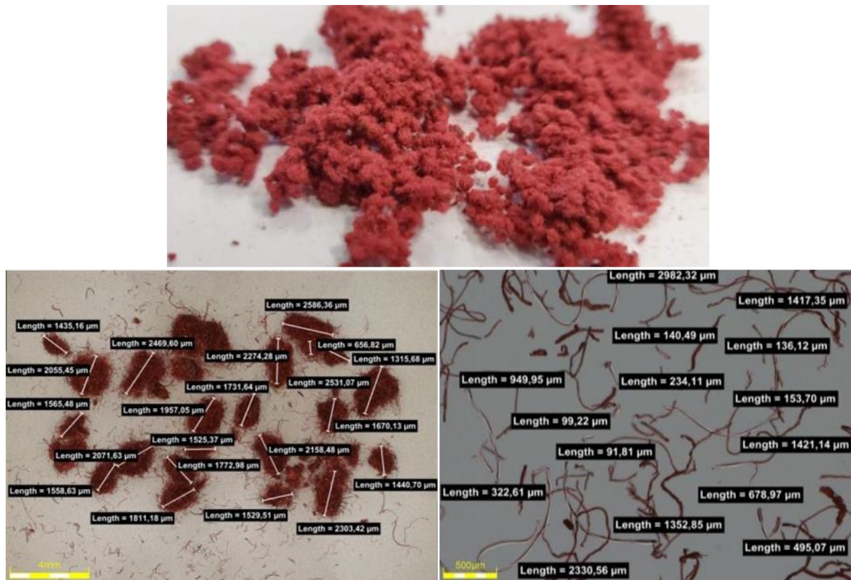
Figure 3 Images of the PES fibres granulated by Procotex including the determination of the granule size and fibre length.
