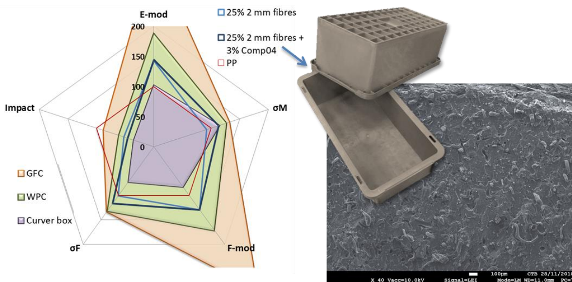
Figure 6 Radar plots comparing the mechanical properties* of the 2 mm mattress fibre-FRC's to unfilled, virgin PP and to virgin WPC and GFC (left) and picture of the final demonstrator as well as a microscope image of the fracture plane of the FRC illustrating the homogeneous distribution of the fibres.
