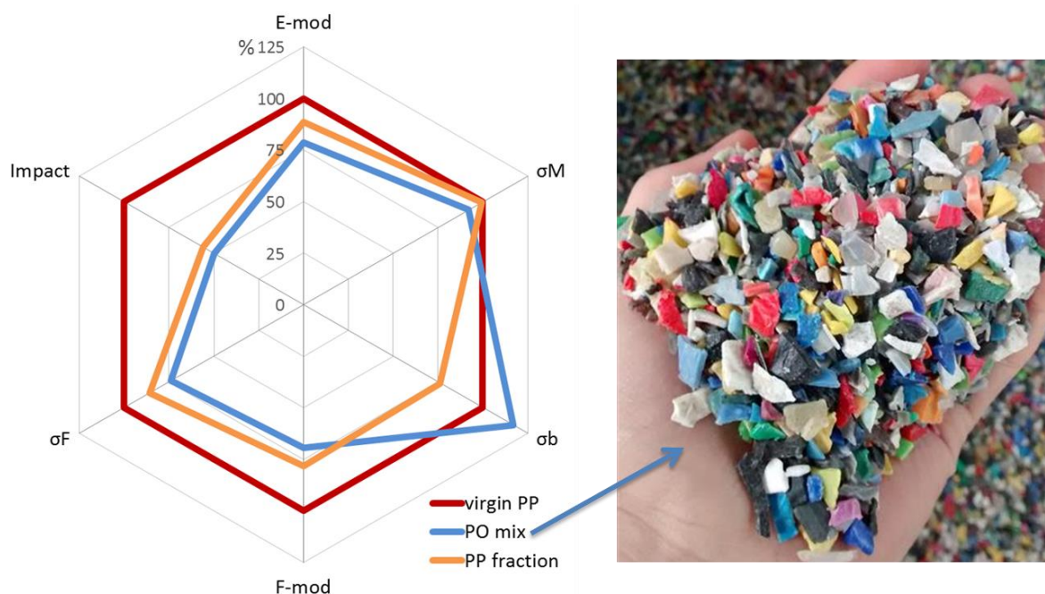
Figure 2 Radar plots comparing the mechanical properties* of the recycled plastics to virgin PP (left) and illustration of the recycled PO mix regrind.
